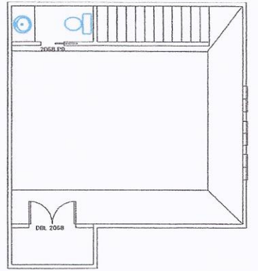
BONUS ROOM 1/4" = 1'
